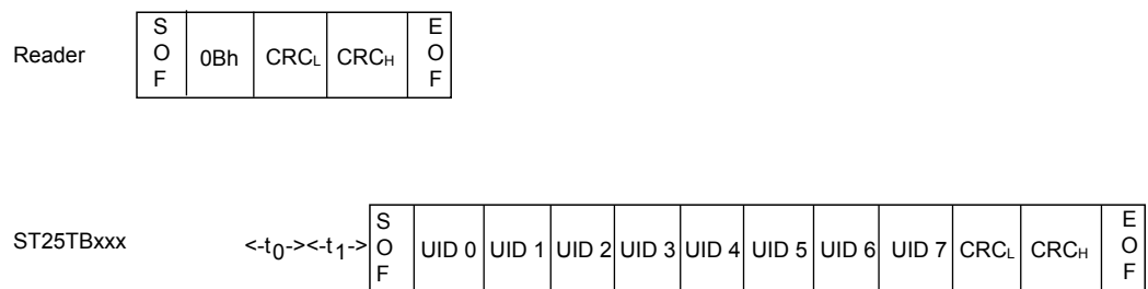
Figure 45. Get_UID frame exchange between reader and ST25TB512-AC
