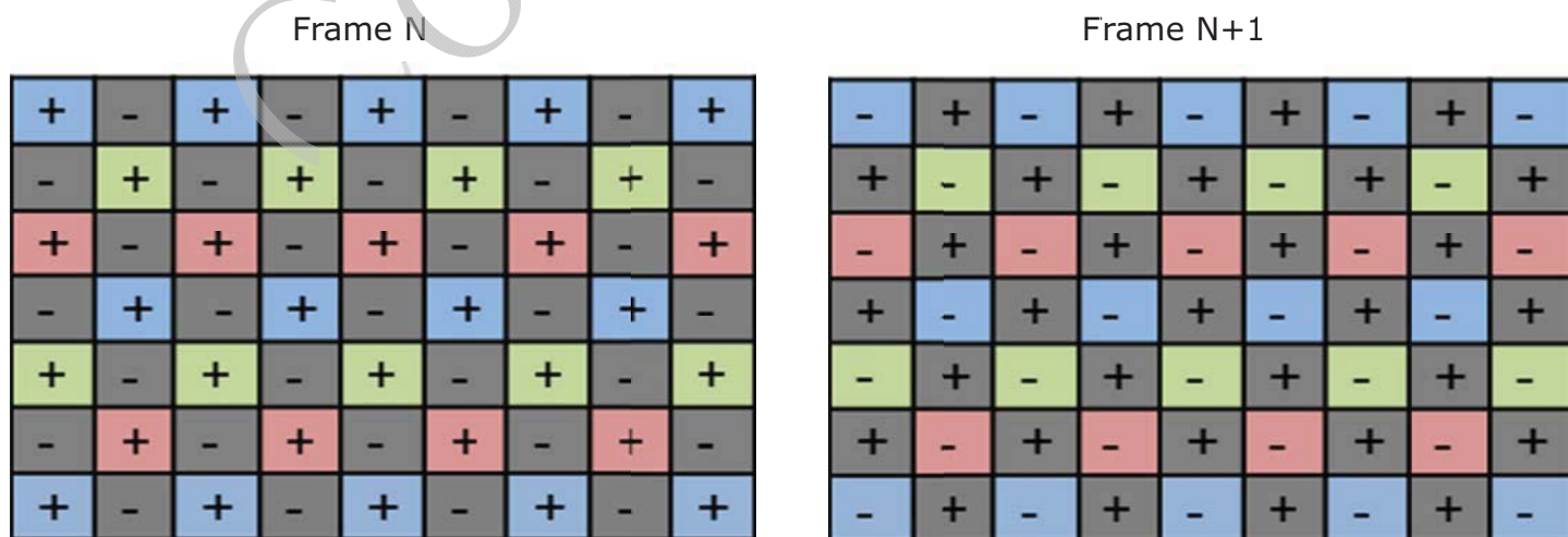
Fig. 4.4 Six pair mode data mapping
