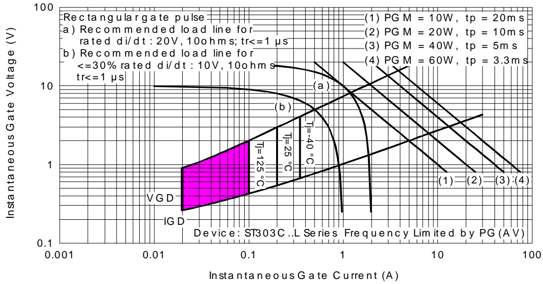
Fig. 17 - Gate Characteristics
