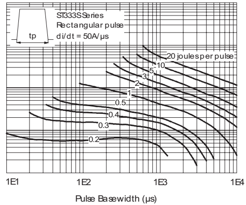
Fig. 14 - Maximum On-State Energy Power Loss Characteristics
