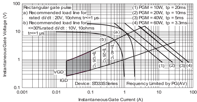
Fig. 15 - Gate Characteristics
