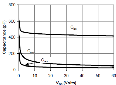
Figure 8: Capacitance Characteristics
