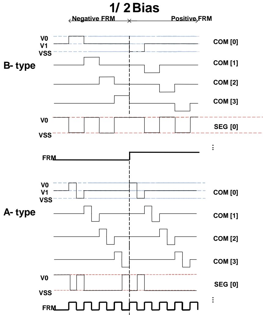
Fig. 18 A-type & B-type of 1/2 Bias waveform
