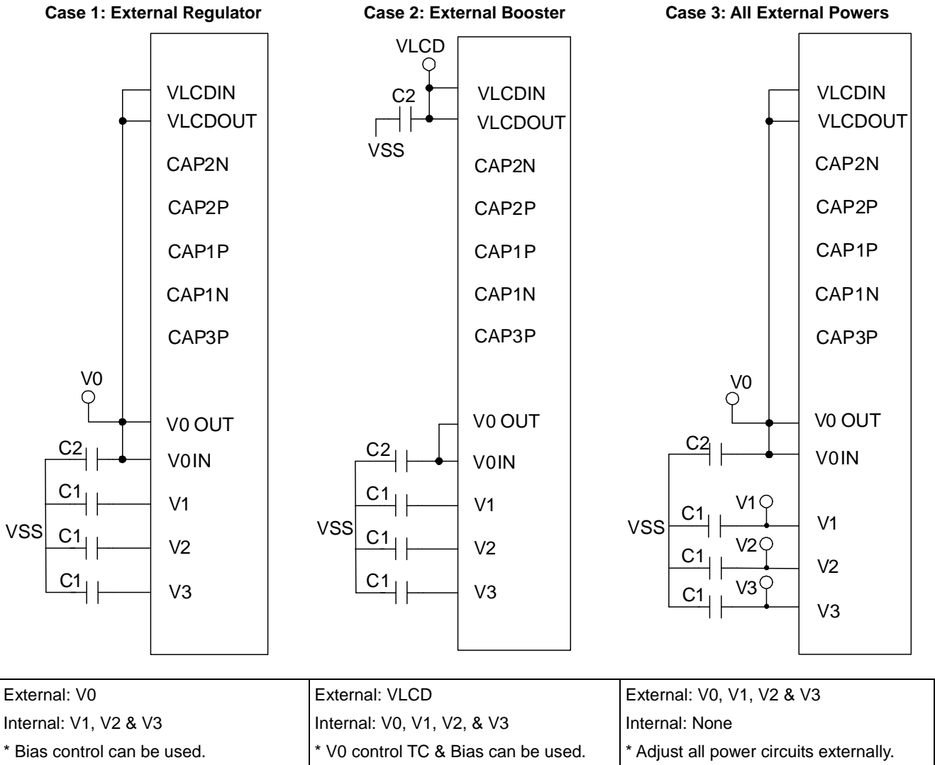
Fig. 14 External Connection for External Power Circuits
