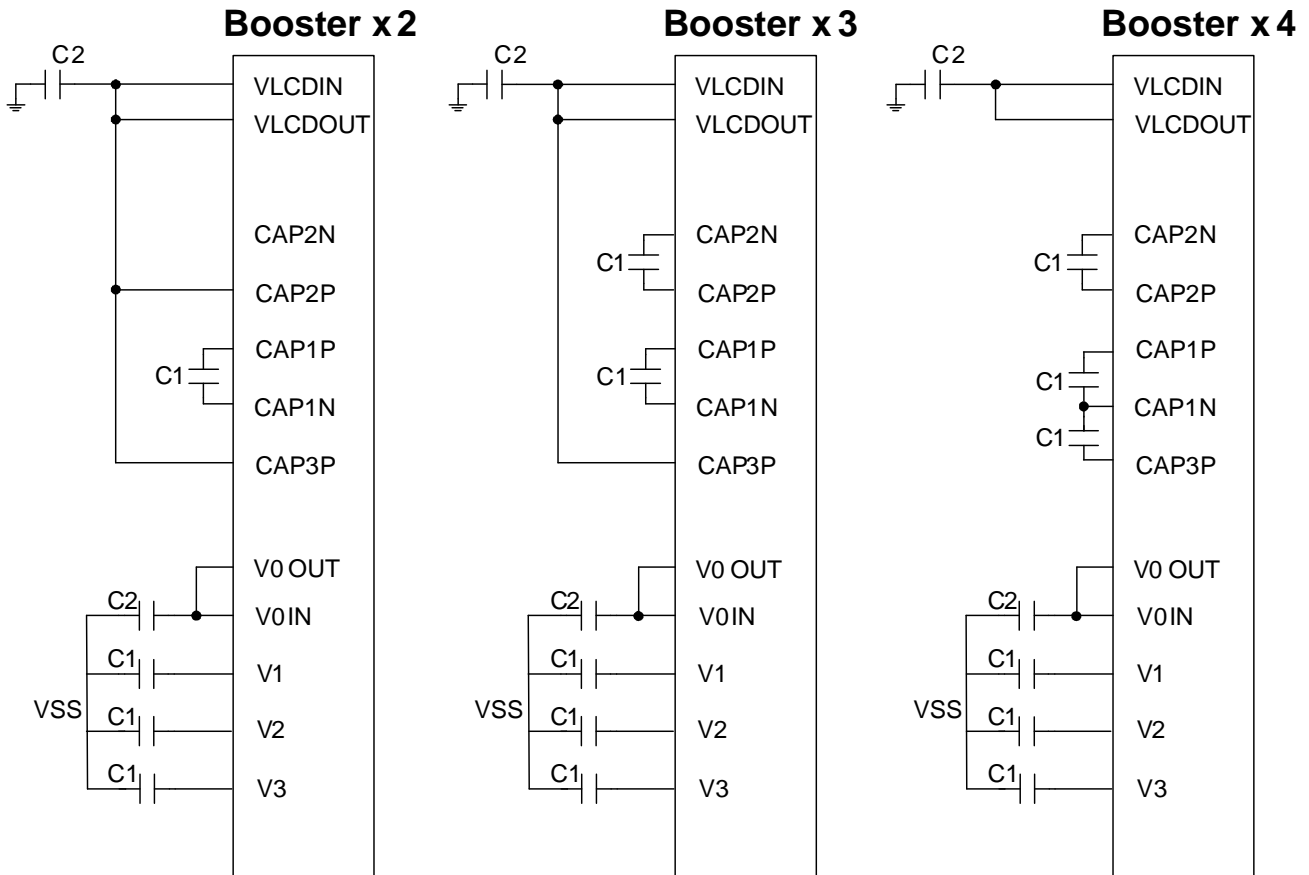
Fig. 13 External Connection for Internal Power Circuits
