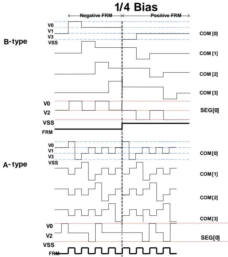
Fig. 20 A-type & B-type of 1/4 Bias waveform
