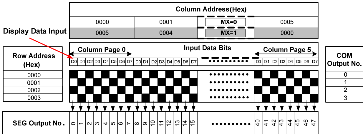
Fig. 11 Data Format and DDRAM Structure
