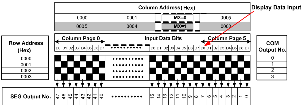
Fig. 12 Transferred DDRAM Map
