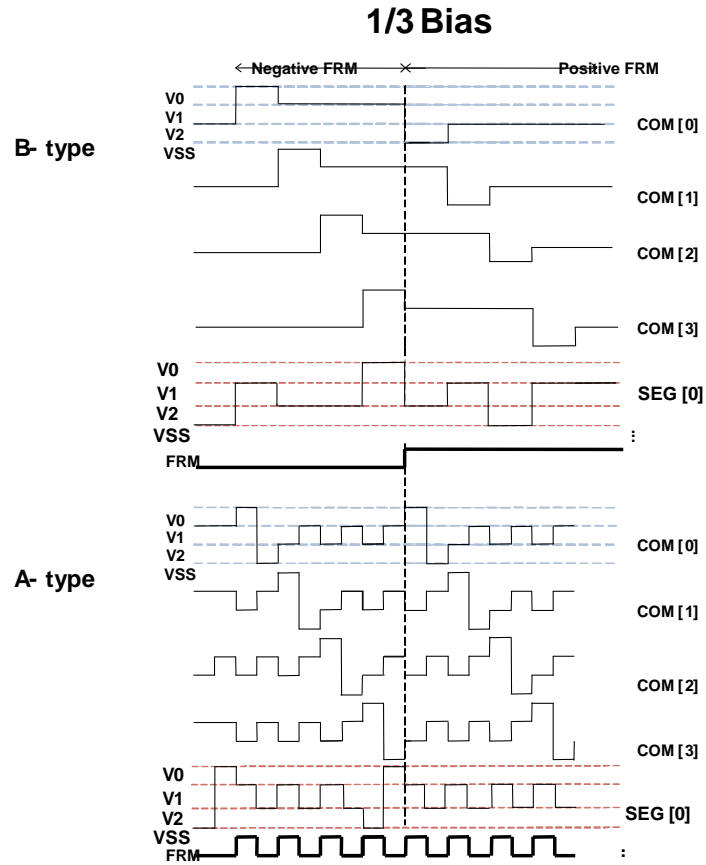
Fig. 19 A-type & B-type of 1/3 Bias waveform
