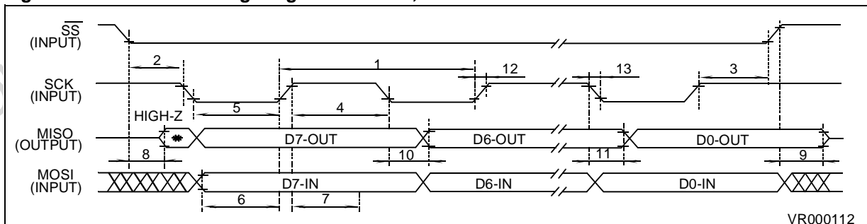
Figure 50. SPI Slave Timing Diagram CPHA=1, CPOL=1
