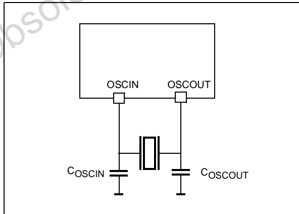
Figure 13. Crystal/Ceramic Resonator
