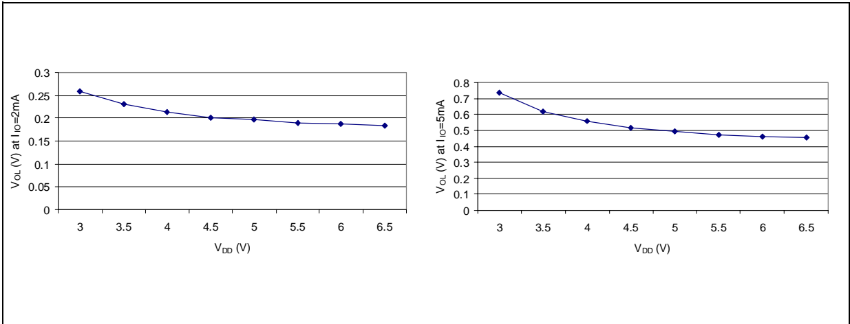
Figure 54. Typical V_{OL} vs. V_{DD} (RESET)
