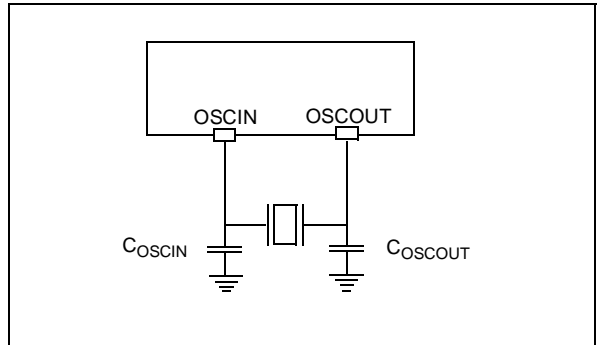
Figure 10. Clock block diagram
