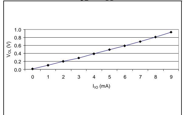
Figure 53. Typical V_{OL} at V_{DD}=5V (RESET)
