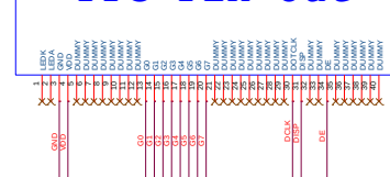
FPC Pin Out
