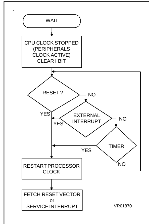
Figure 15. WAIT Flow Chart
