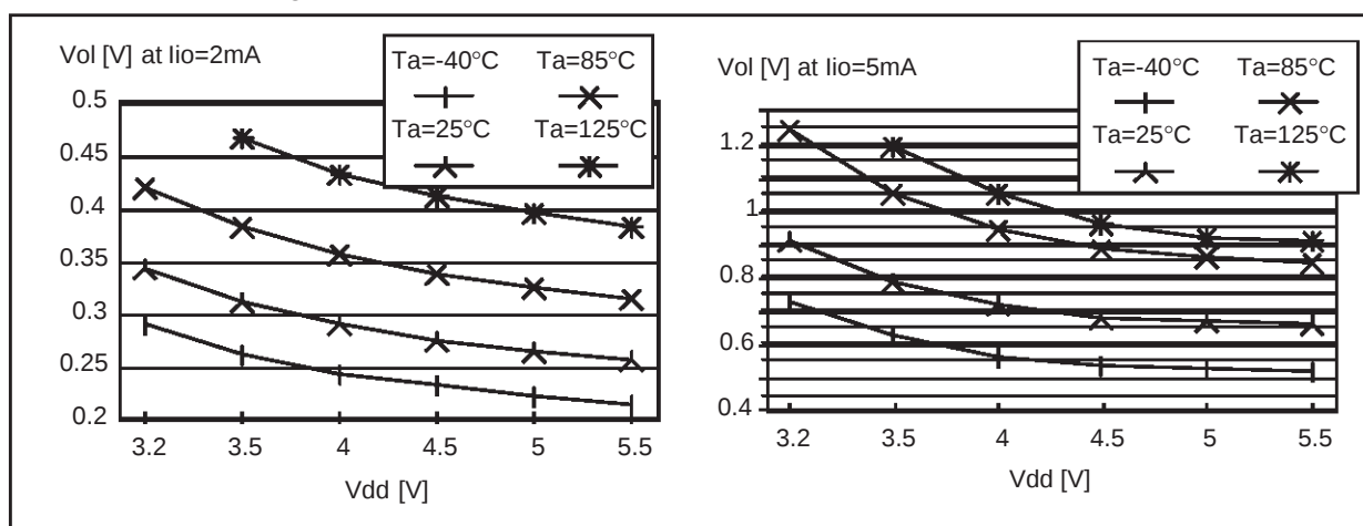
Figure 89. Typical V_{OL} vs. V_{DD} ( \overline{\text{RESET}} )
