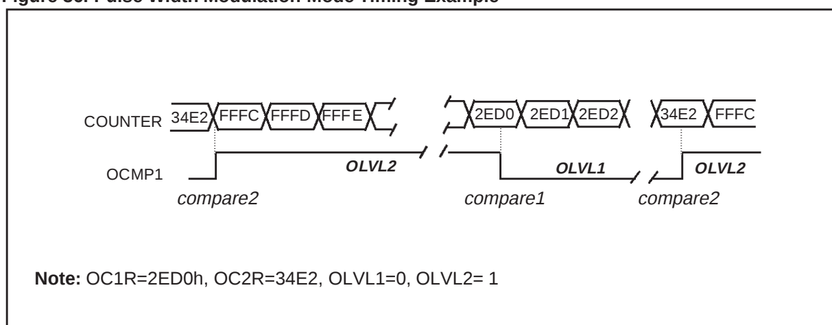
Figure 36. Pulse Width Modulation Mode Timing Example
