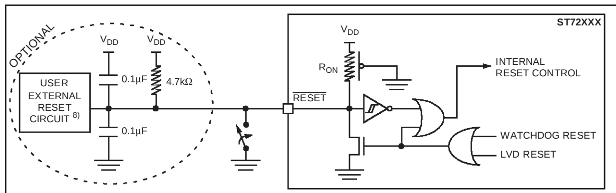
Figure 86. Typical Application with RESET pin 8)
