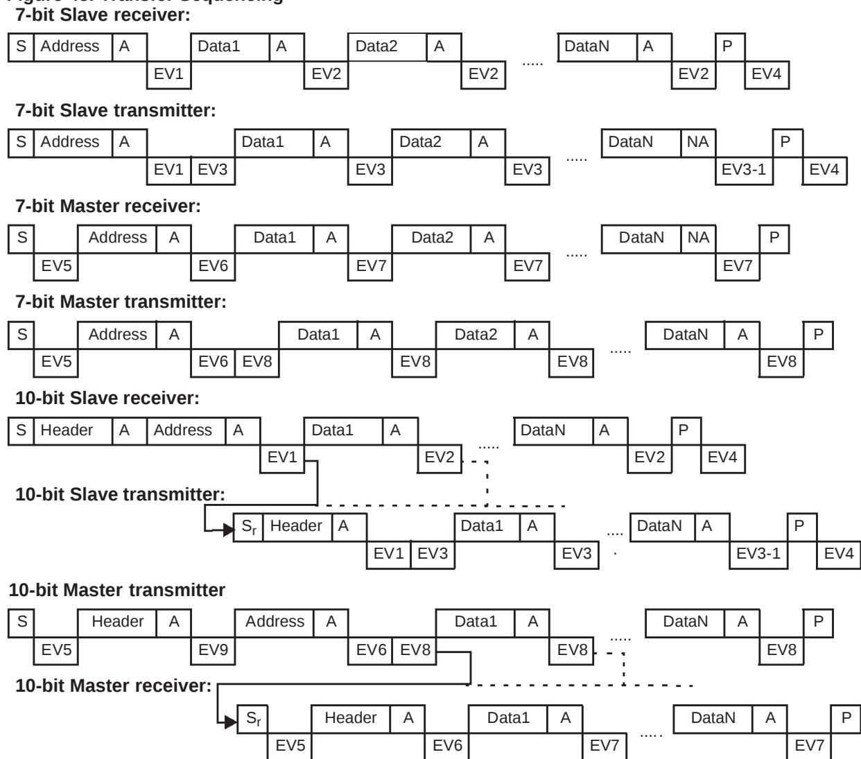
Figure 45. Transfer Sequencing
