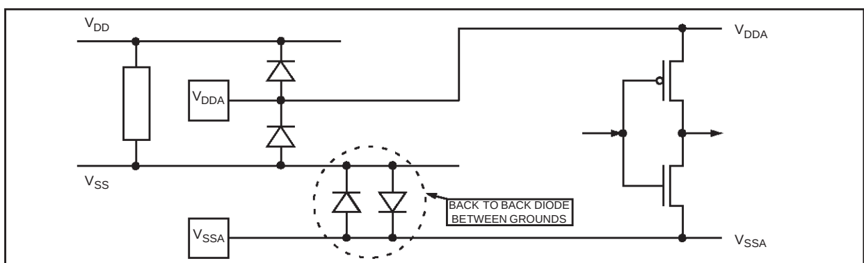
Figure 77. Multisupply Configuration
