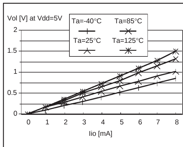
Figure 88. Typical V_{OL} at V_{DD}=5\text{V} ( \overline{\text{RESET}} )
