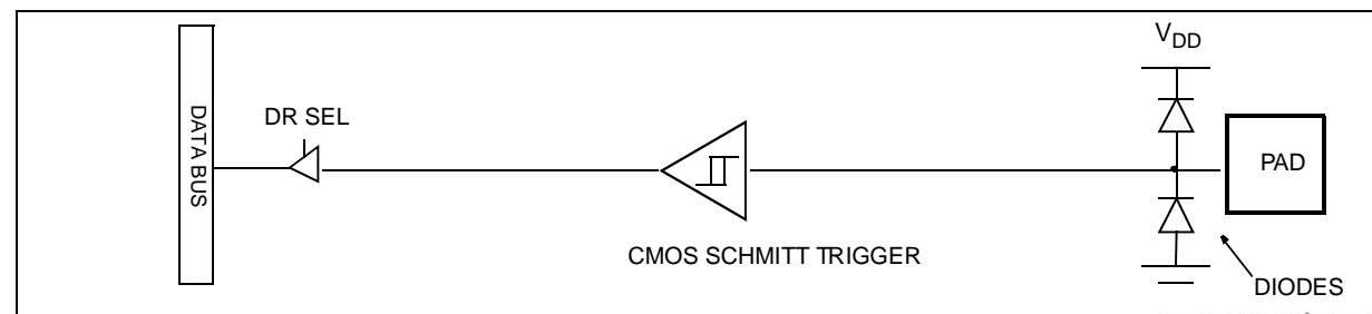
Figure 22. PA6 Configuration
