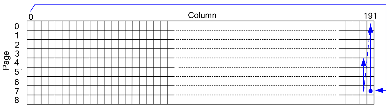
Fig 27. DDRAM Access Mapping (MX=1, AC[2:0]=7, PA[3:0]=7, CA[3:0]=0)
