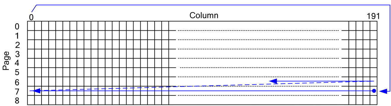
Fig 25. DDRAM Access Mapping (MX=1, AC[2:0]=5, PA[3:0]=7, CA[3:0]=0)
