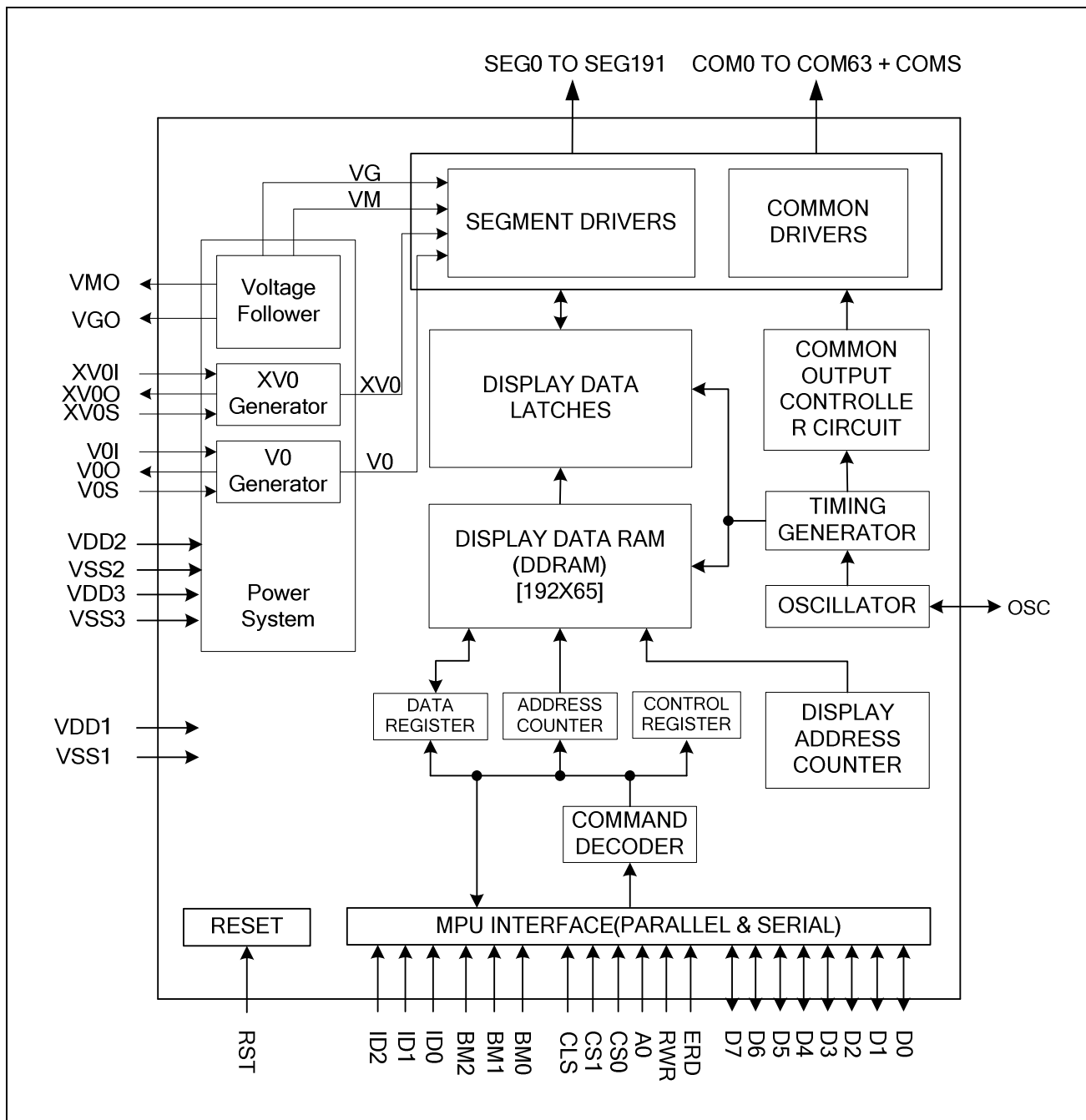
Fig 2. Block Diagram
