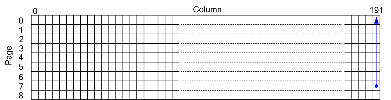
Fig 26. DDRAM Access Mapping (MX=1, AC[2:0]=6, PA[3:0]=7, CA[3:0]=0)
