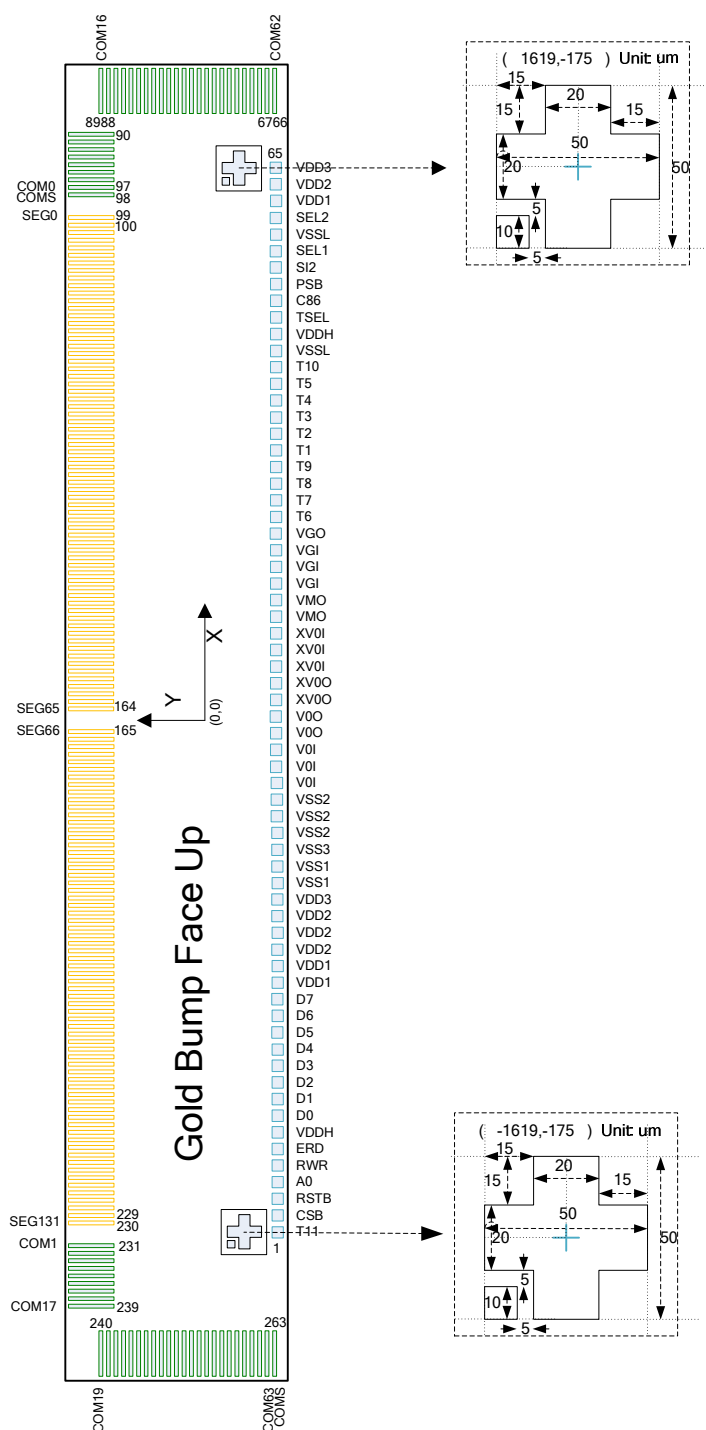
Figure 1 Chip Outline
