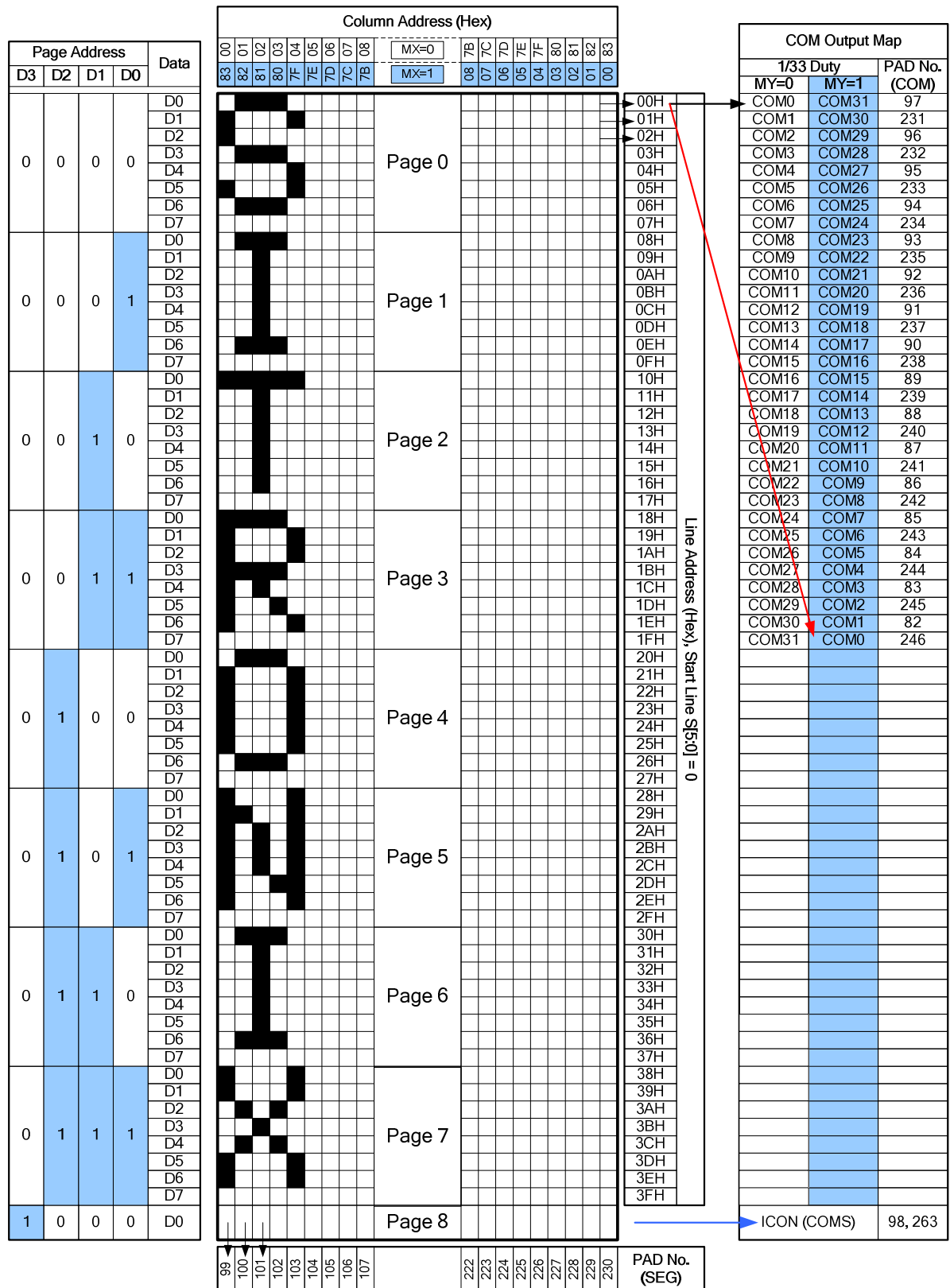
Figure 16 DDRAM and Output Map (COM/SEG) 1/33 Duty
