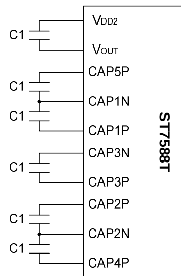
6x step-up voltage circuit
