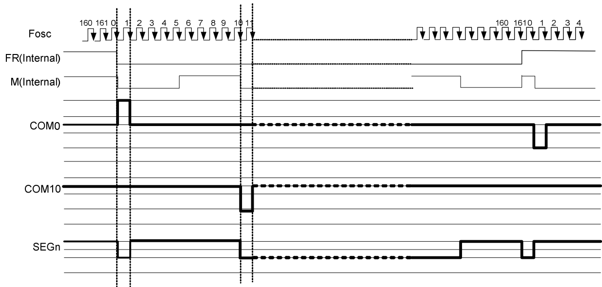
Figure 7.3-4 N-Line Inversion Driving Waveform (N=10, Duty Ratio=1/162)
