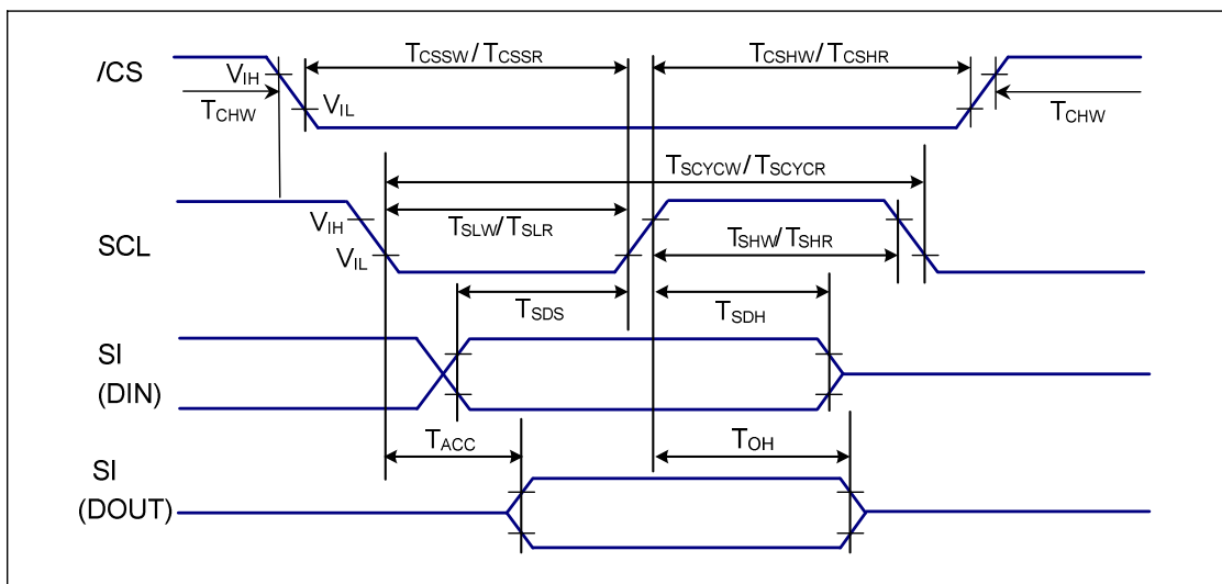
Figure 7.10.2-1 3-pin Serial Interface Characteristics
