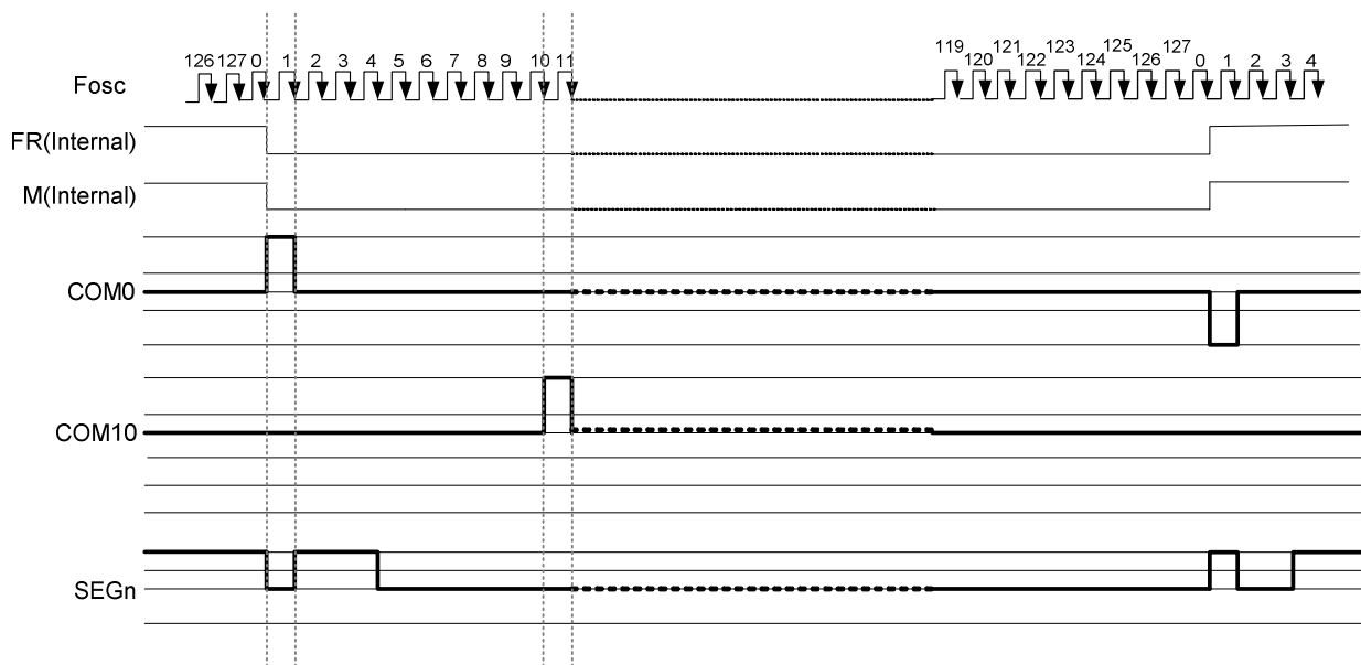
Figure 6 2-frame AC Driving Waveform (Duty Ratio: 1/128)
