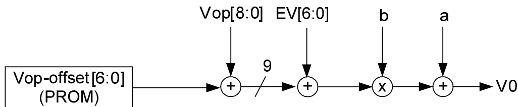
Figure 10 V0 value control for different modules by loading PROM offset
