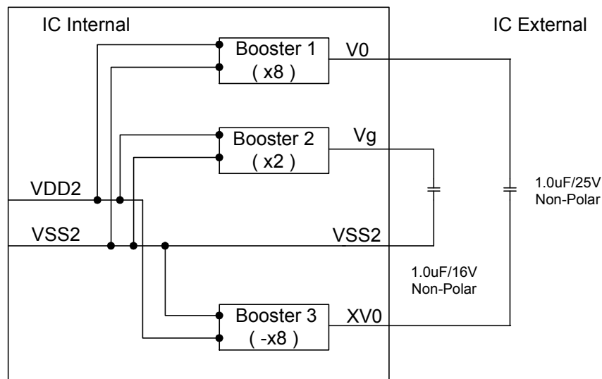
Figure 8 DC/DC Booster Block Diagram
