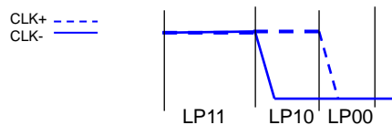
Figure 5.9: From LPM mode to ULPM
