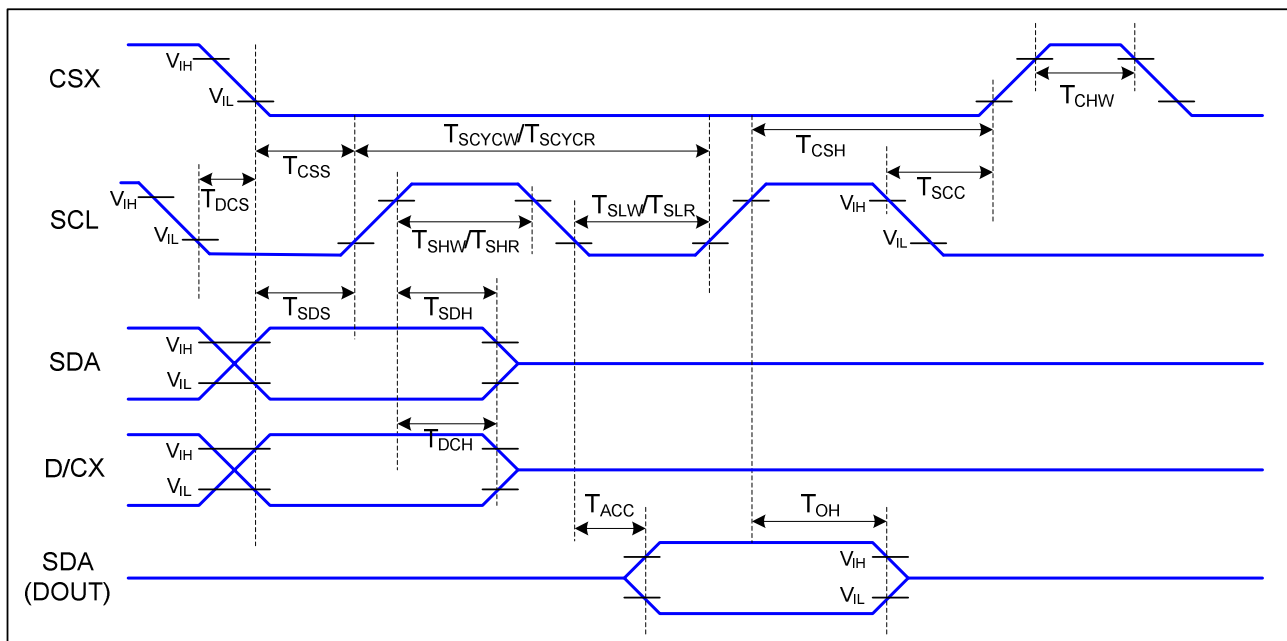
Figure 8.4.1 4-line serial interface timing
