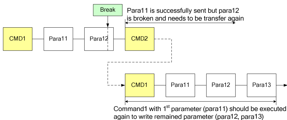
Figure 9.5.3 Write interrupts recovery (serial interface)
