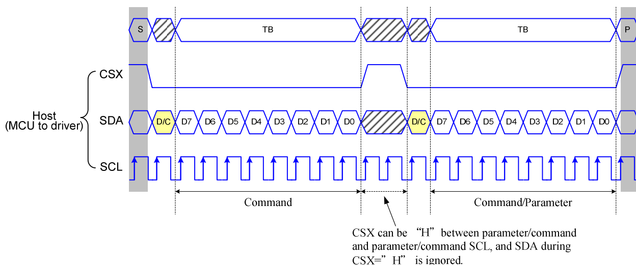
Figure 9.4.3 3-line serial interface write protocol (write to register with control bit in transmission)
