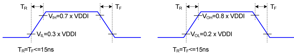
Figure 8.1.2 Rising and falling timing for input and output signal
