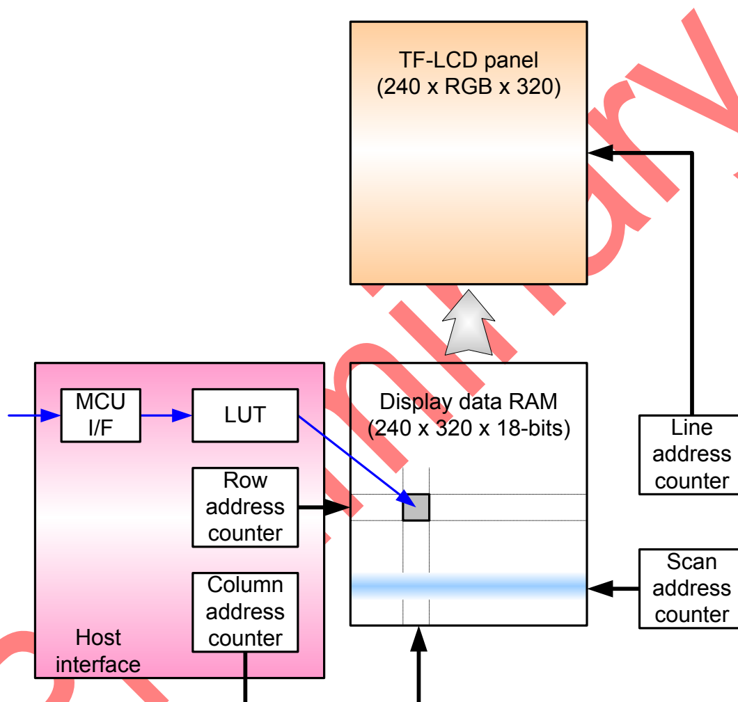
Figure 32 Display data RAM organization
