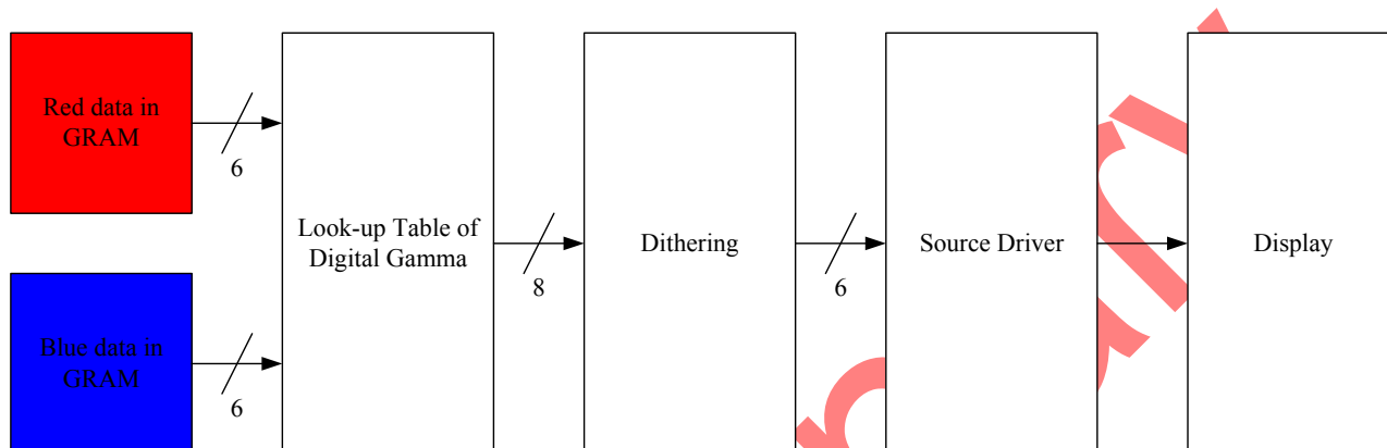
Figure 37 Block diagram of digital gamma
