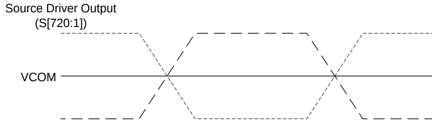
Figure 36 Relationship between Source Output and VCOM
