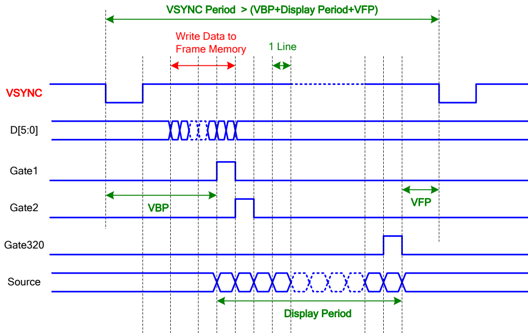
Figure 29 Timing Diagram of VSYNC Interface
