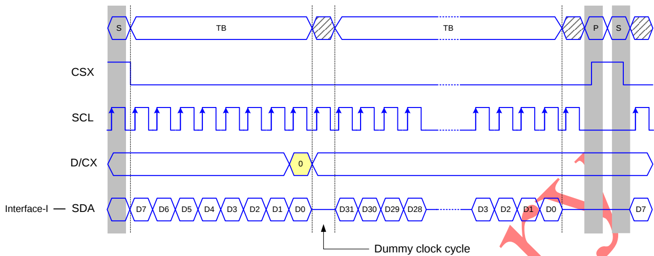
Figure 16 4-line serial interface read protocol
