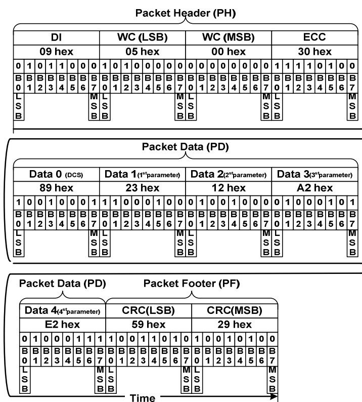
Null Packet, No Data (NP-L)-Example
