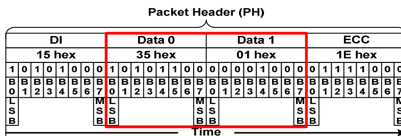
Packet Data (PD) for Short Packet (SPa), 2 Bytes Information
