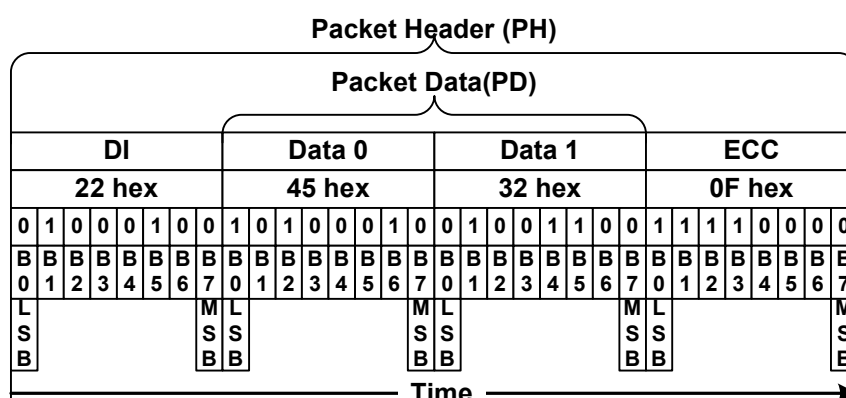
DCS Read Short Response, 2 Bytes Returned (DCSRR2-S) –Exmpl
