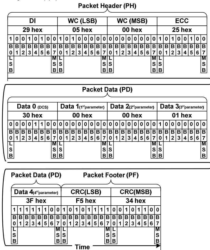
Generic Write Long (GENW-L) with DCS and 4 Parameters-Example
