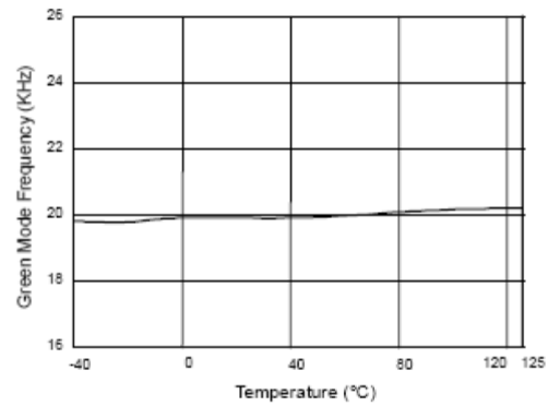
Fig. 4 Green Mode Frequency vs. Temperature
