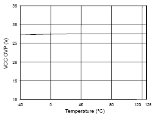
Fig. 10 VCC OVP vs. Temperature
