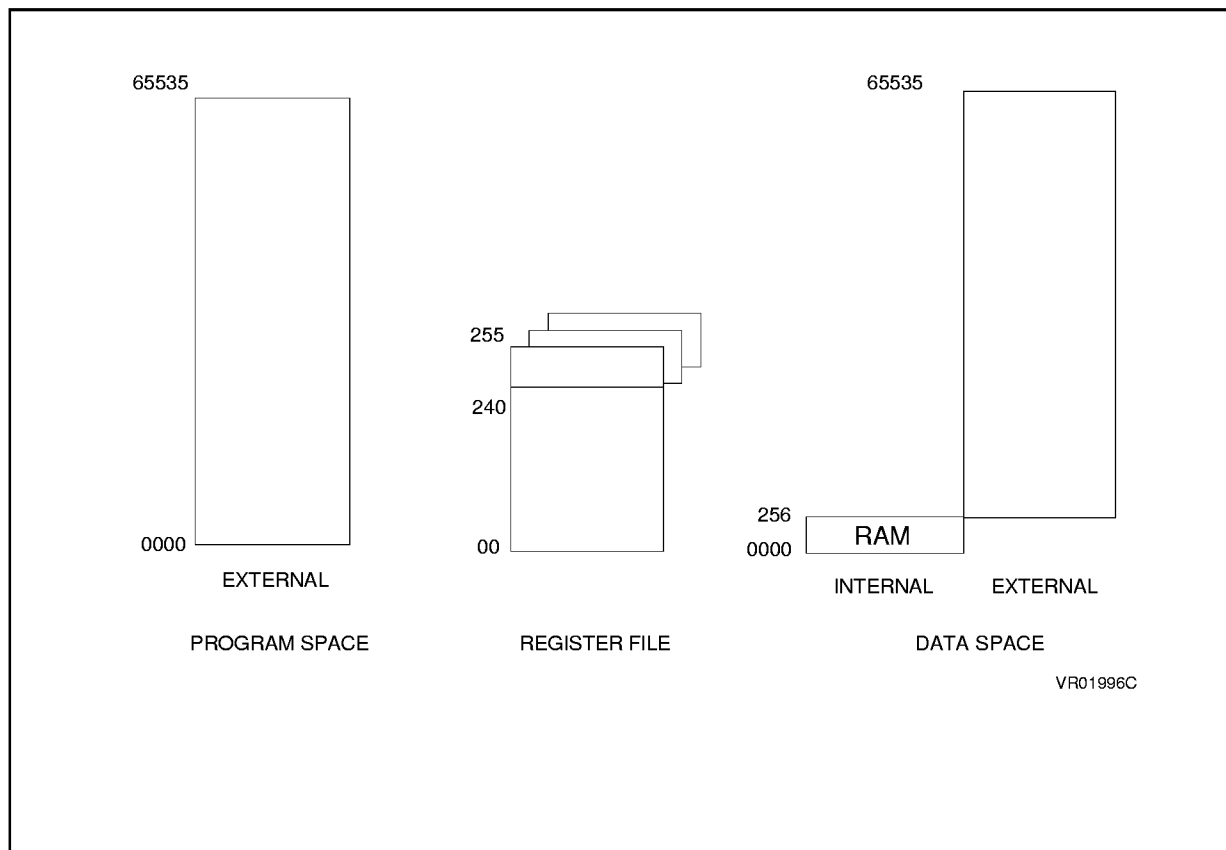
Figure 1-3. Memory Spaces
