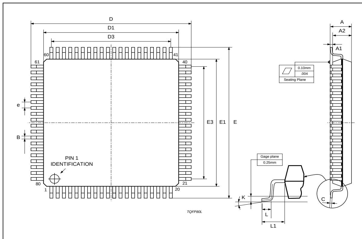
TQFP80 (14x14x1.40mm)
