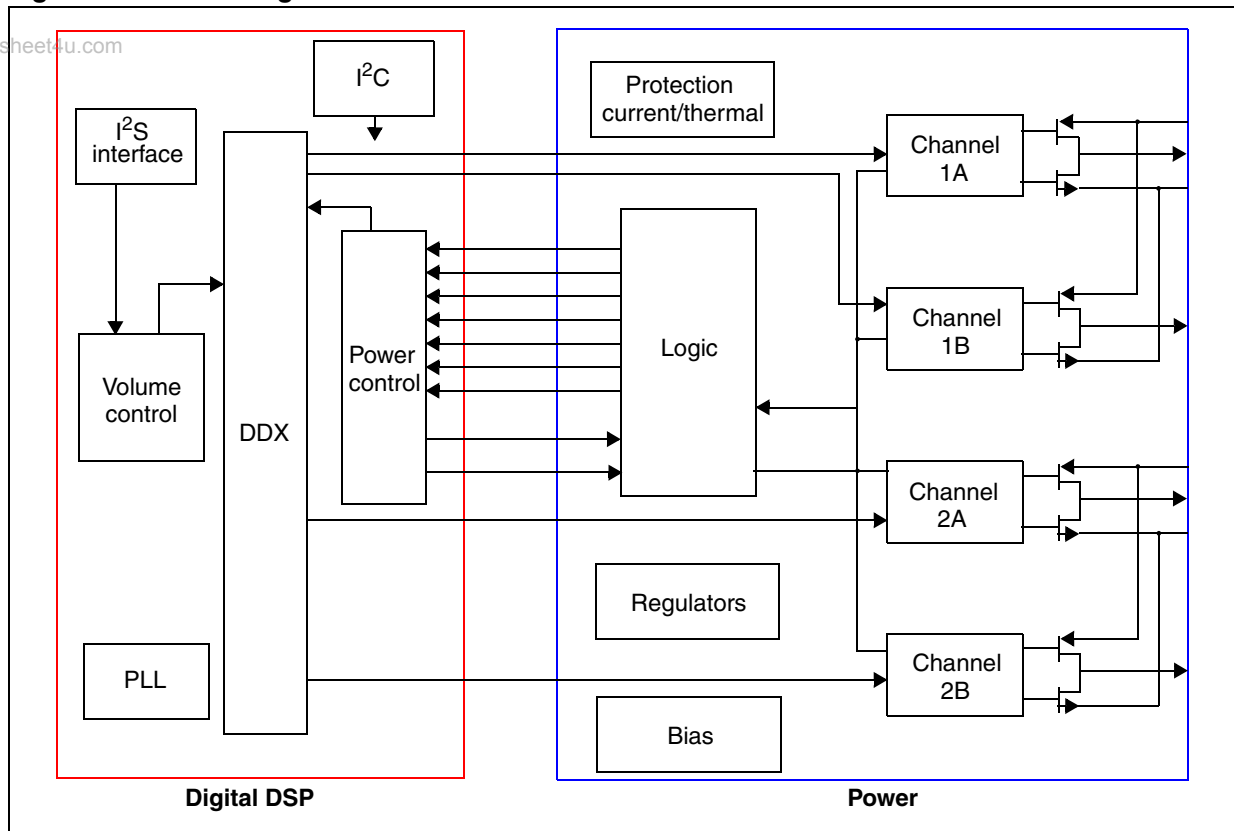
Figure 2. Block diagram
