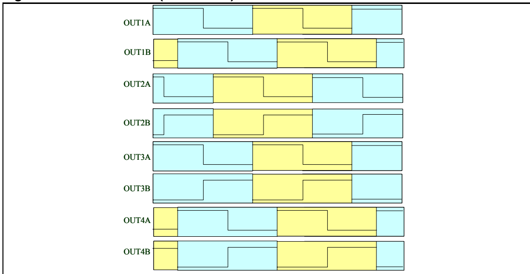
Figure 14. 2.1 channels (OCFG = 01) PWM slots
