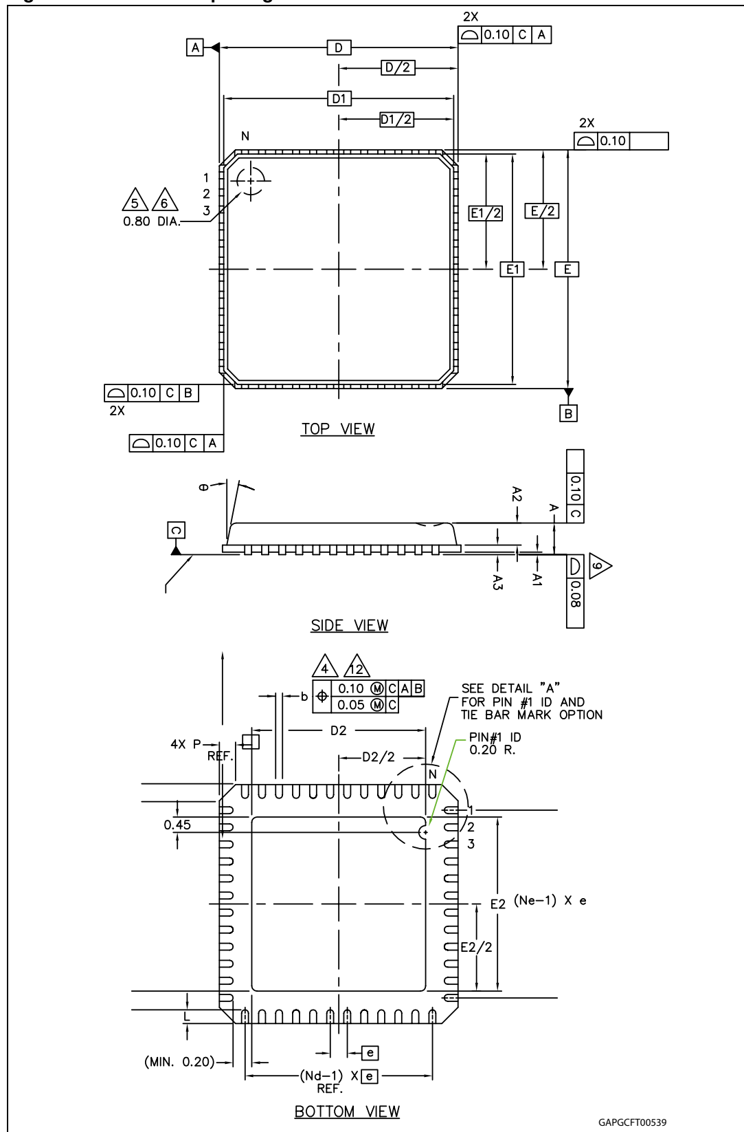
Figure 4. VFQFPN56 package dimension
