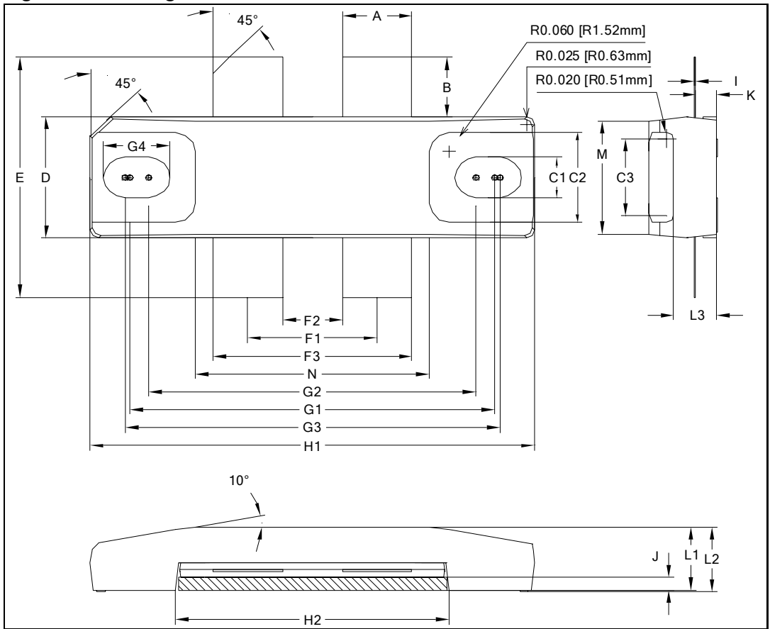
Figure 11. Package dimensions
