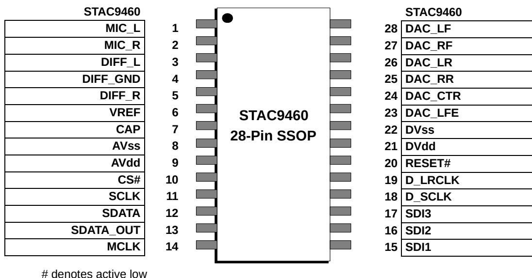
Figure 9. STAC9460 Pin Designation
