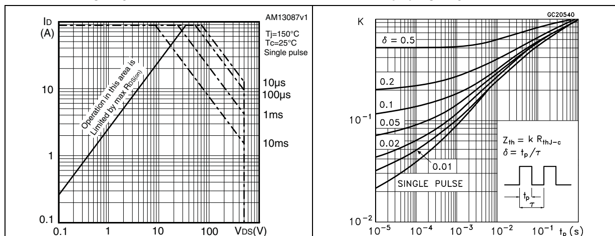
Figure 2. Safe operating area for D 2 PAK and TO-220 Figure 3. Thermal impedance for for D 2 PAK and TO-220
