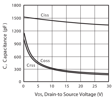
Figure 9. Capacitance
