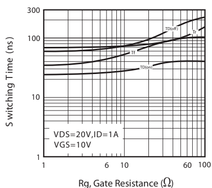
Figure 11. Switching Characteristics
