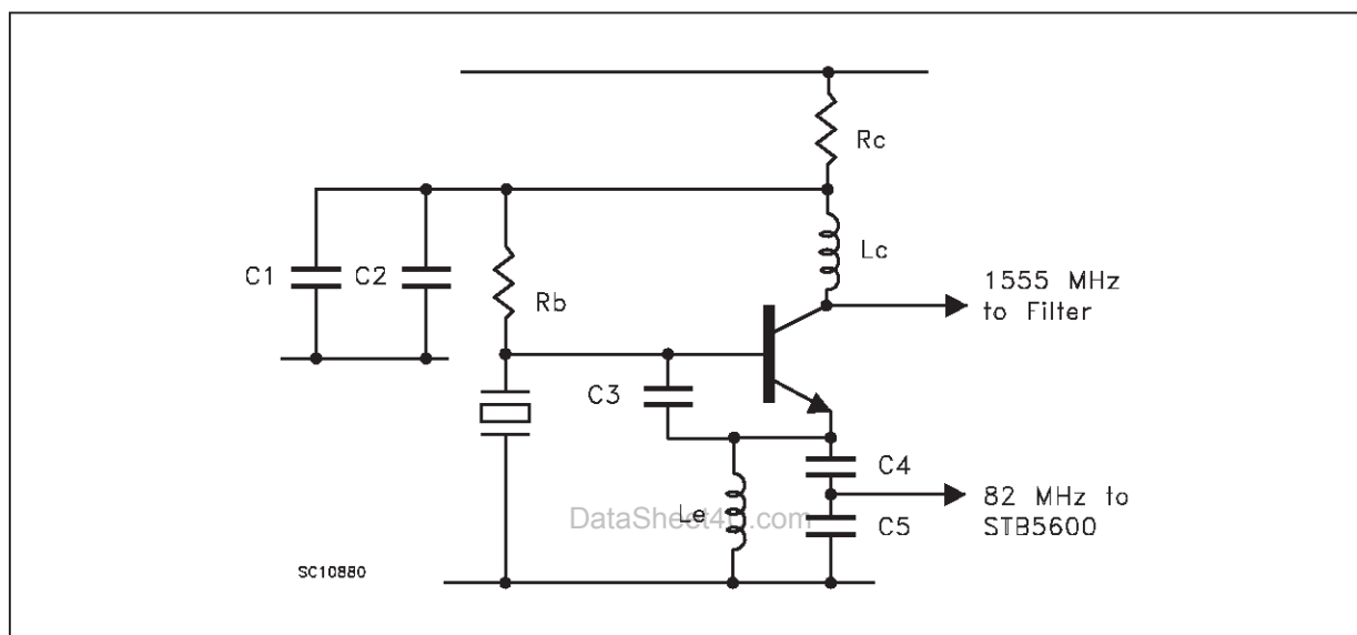
Fig. 6 Reference Oscillator
