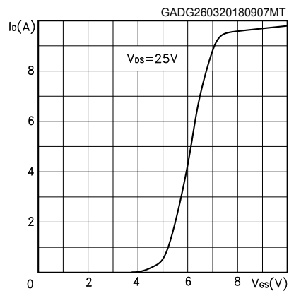
Figure 8. Transfer characteristics
