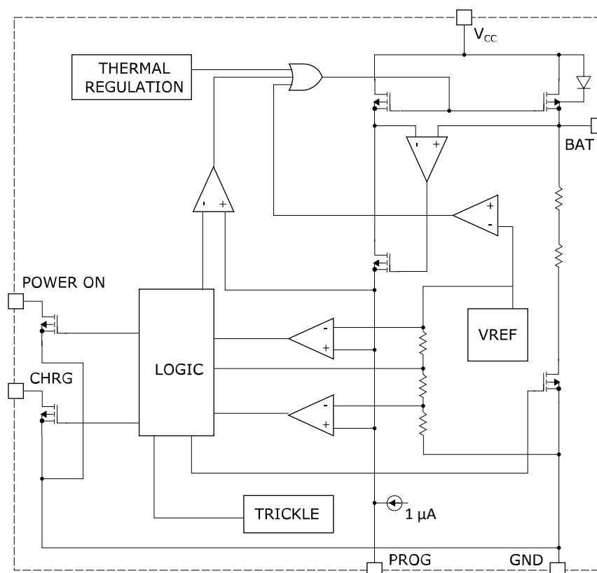
Figure 1. Block diagram
