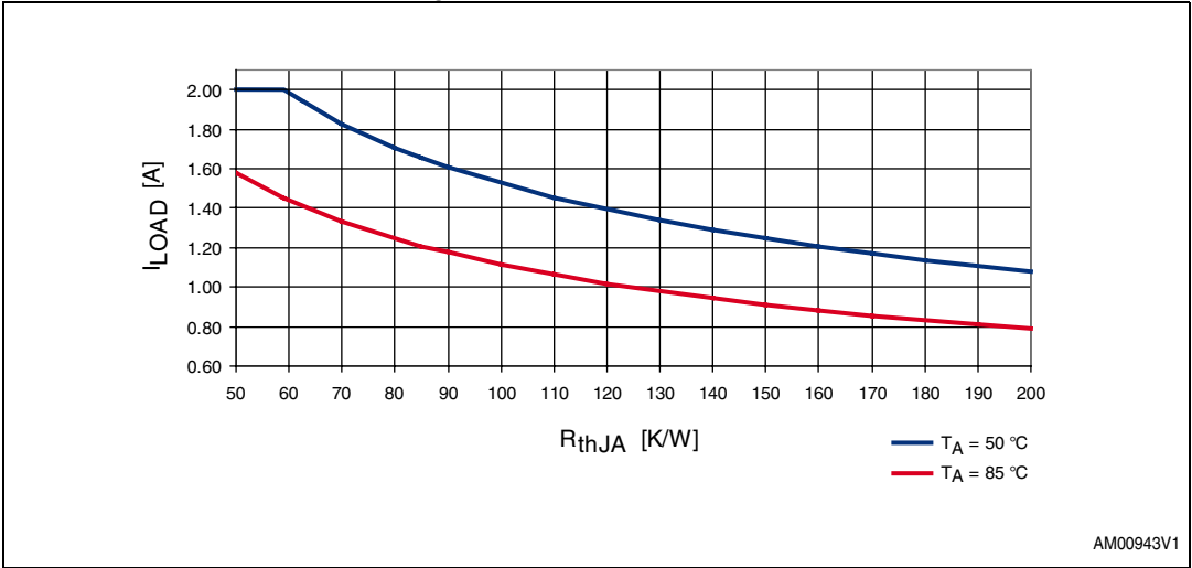
Figure 9. Maximum load current at T_A = 50\text{ }^{\circ}\text{C} and 85\text{ }^{\circ}\text{C} for various PCB thermal performance and T_J \leq 125\text{ }^{\circ}\text{C}
