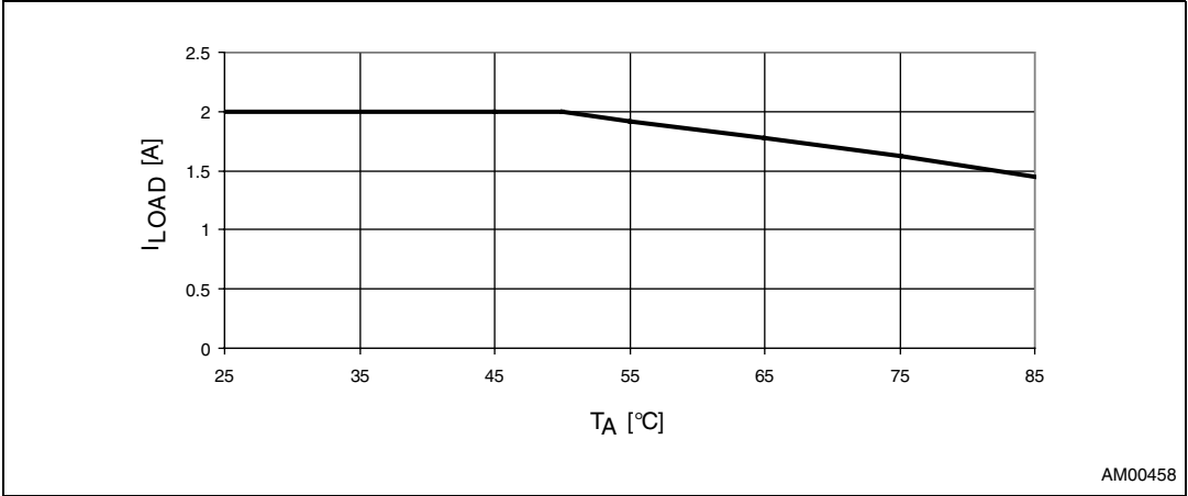
Figure 10. Maximum load current vs. ambient temperature for R_{thJA} = 59\text{ K/W} and T_J \leq 125\text{ }^{\circ}\text{C}
