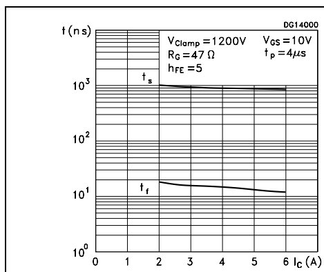
Figure 9. Inductive load switching time
