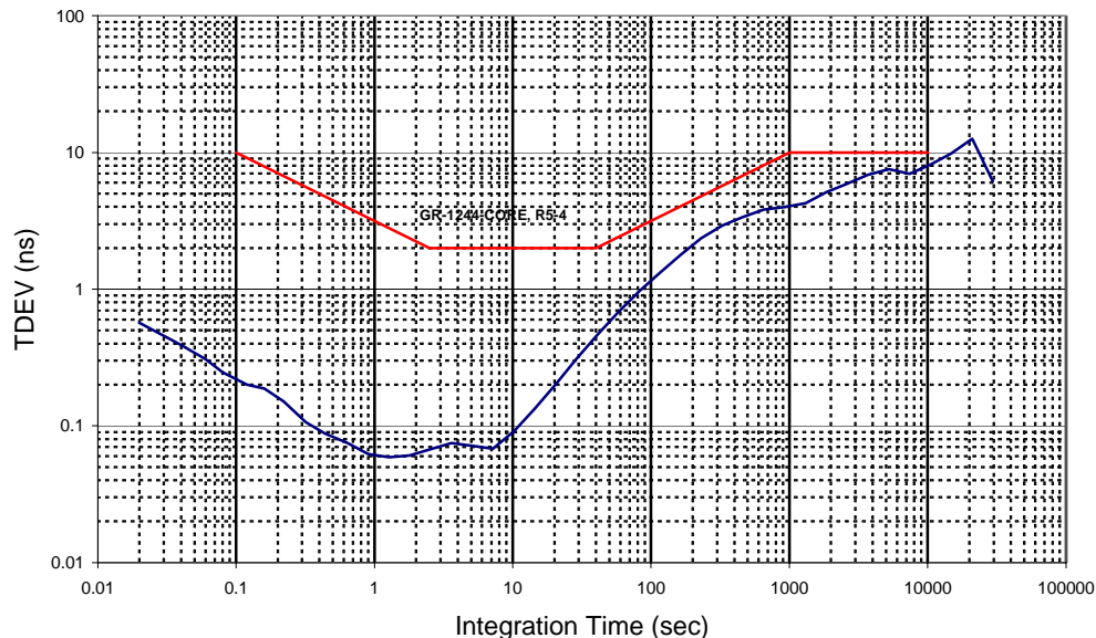
Wander Generation Characteristics – TDEV (10 Hz single-pole LPF applied)
