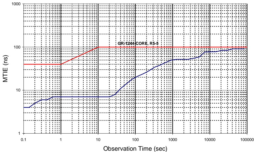
Wander Generation Characteristics – MTIE (10 Hz single-pole LPF applied)
