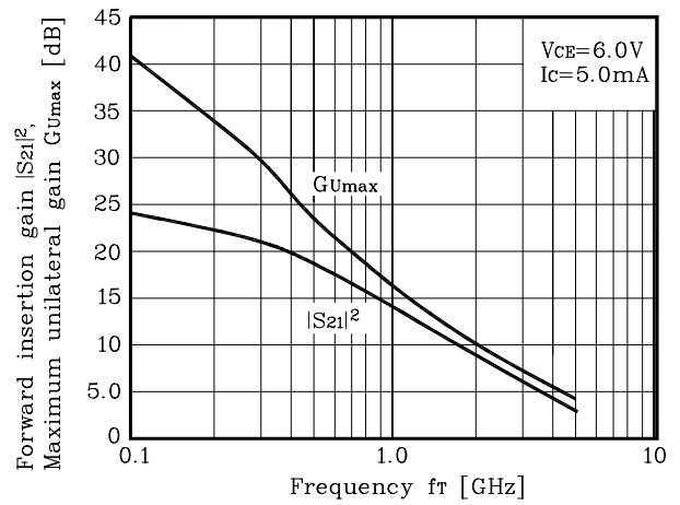
Fig. 9 |S_{21}|^2, G_{Umax} -f T
