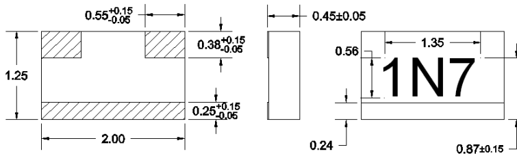
Planar Configuration
