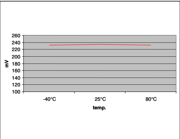
Figure 19. V_{FB2} vs Temp. at I_O = 800\text{mA} , V_1 = 3.3\text{V}
