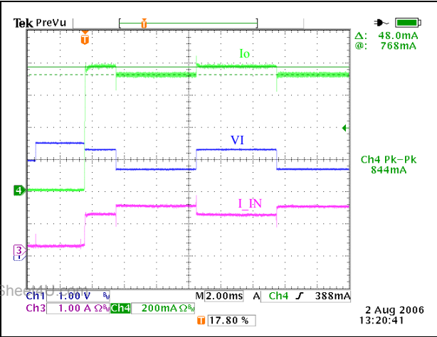
Figure 22. Line transient in Flash Mode 800mA, change of V_I from 2.7V to 3.3V in 10μs
