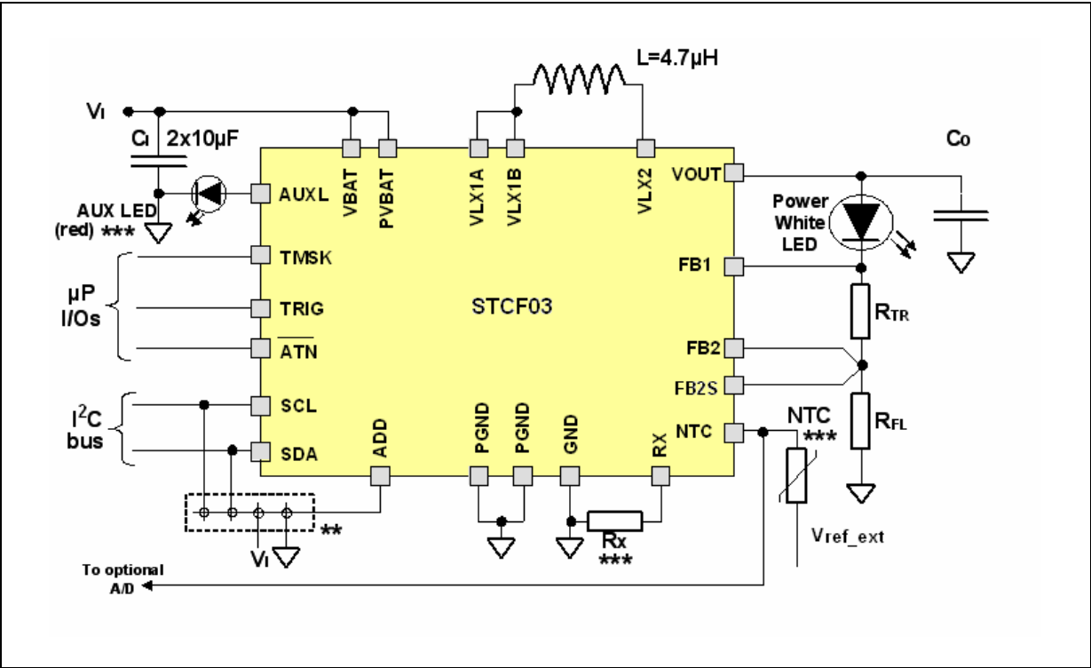
Figure 3. Application schematic
