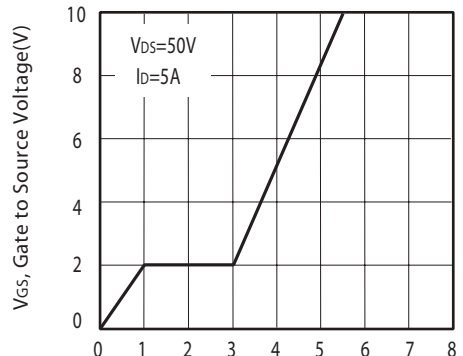
Figure 10. Gate Charge
