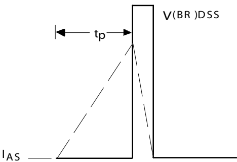
Uncamped Inductive Waveforms
