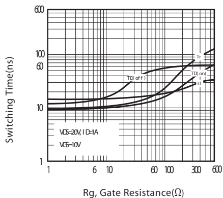
Figure 11. switching characteristics
