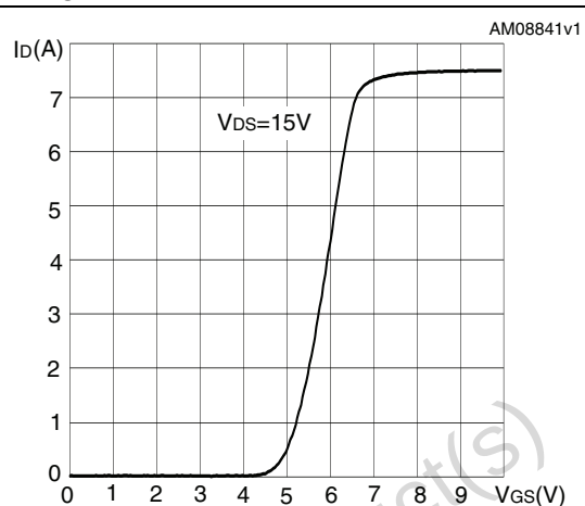
Figure 9. Transfer characteristics
