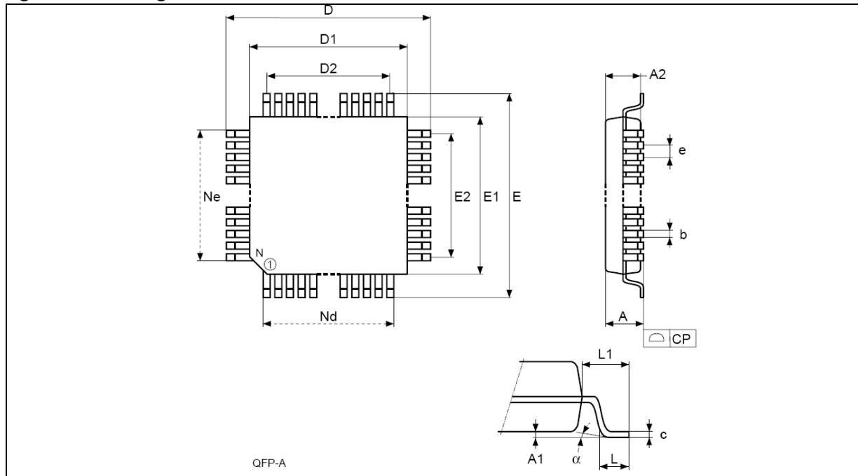
Figure 34. Package dimensions
