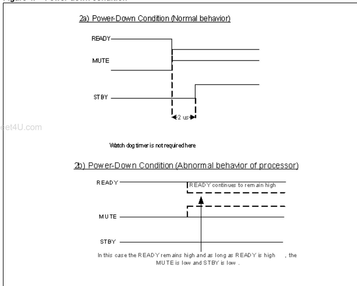
Figure 4. Power-down condition
