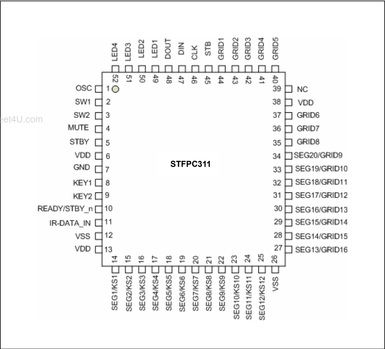
Figure 2. Connection diagram (top view PQFP-52)
