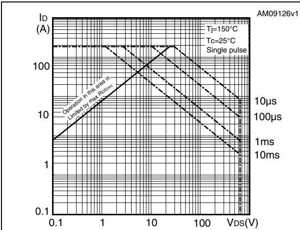
Figure 2. Safe operating area for TO-3FP
