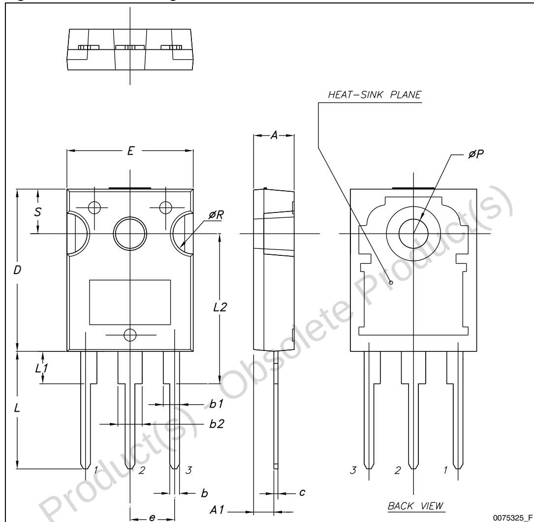
Figure 23. TO-247 drawing
