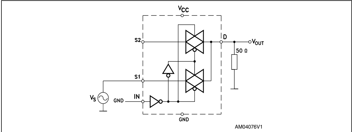
Figure 8. OFF-isolation
