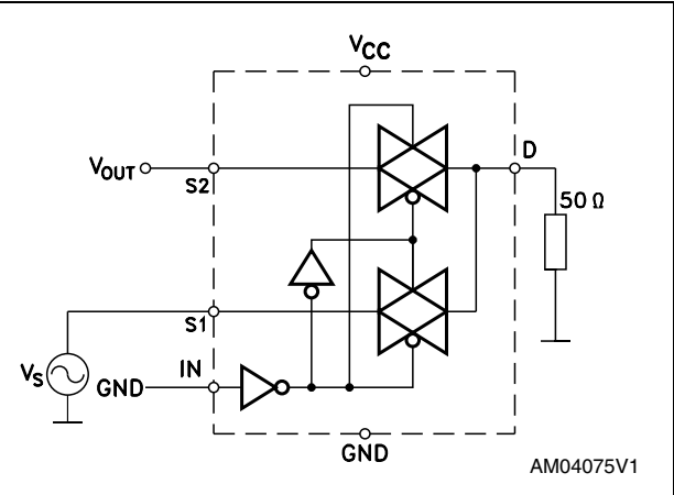
Figure 7. Channel-to-channel crosstalk
