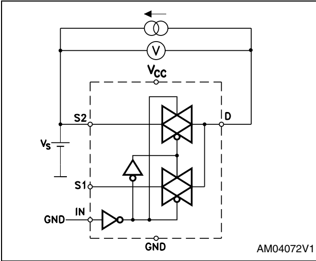
Figure 6. OFF leakage
