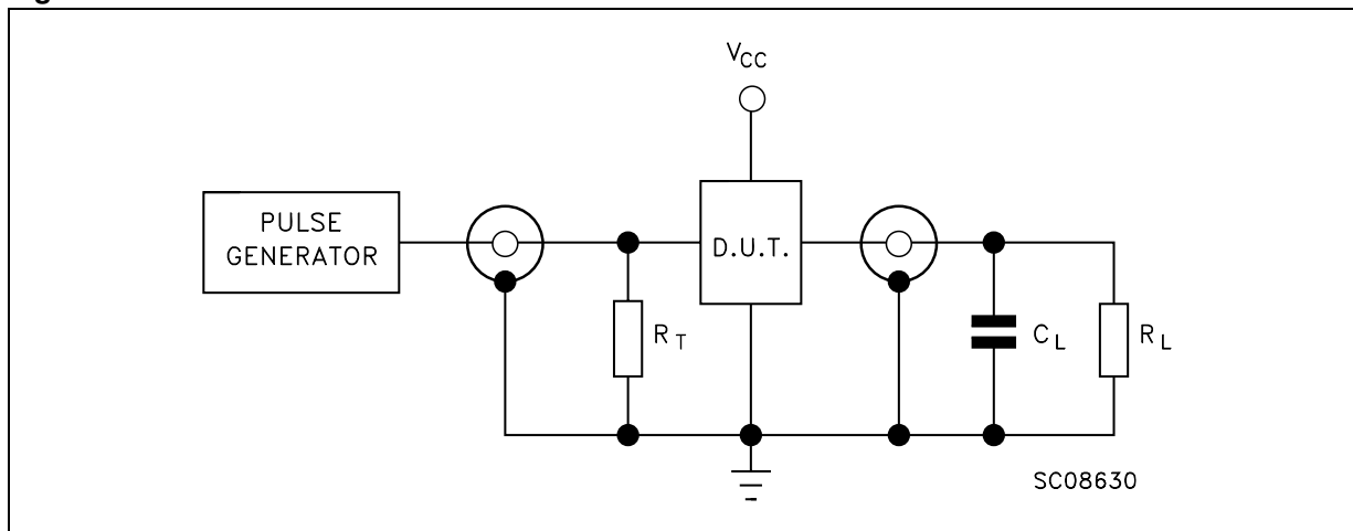
Figure 9. Test circuit
