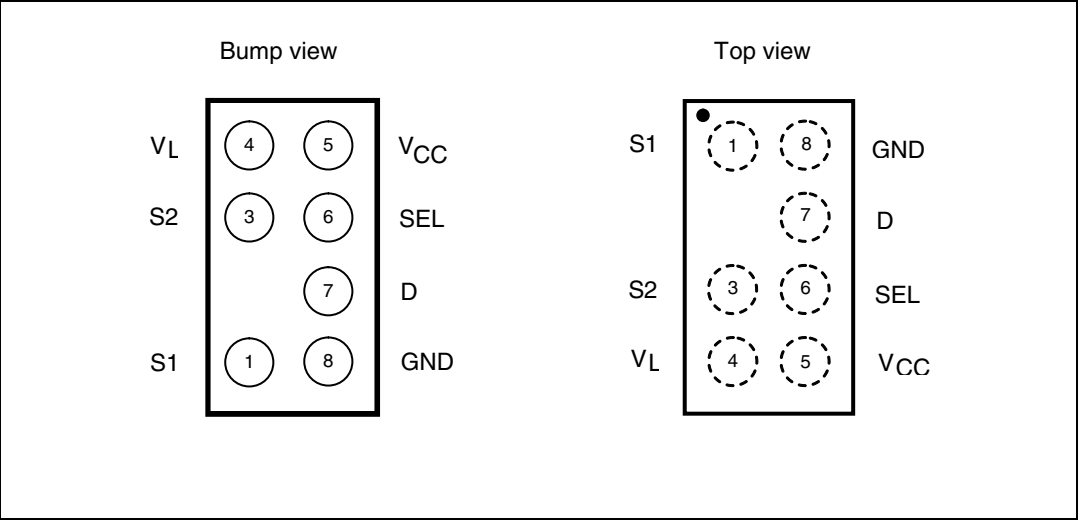
Figure 3. Pin connections
