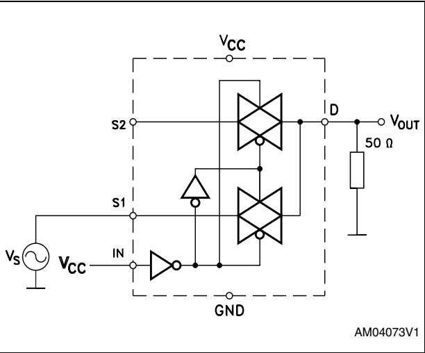
Figure 7. Channel-to-channel crosstalk
