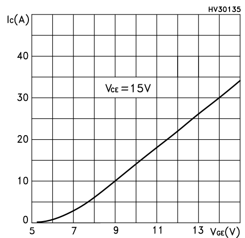
Figure 12. Transfer characteristics
