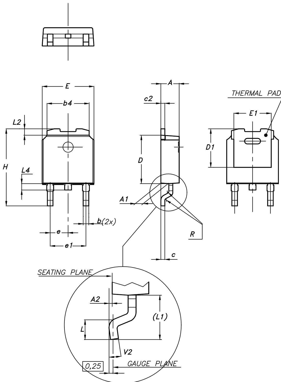
Figure 20. DPAK (TO-252) type A2 package outline
