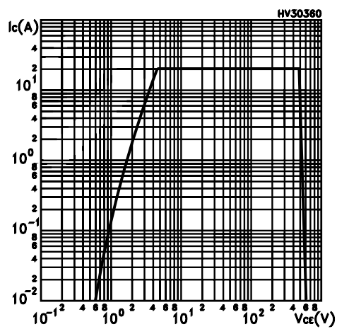
Figure 14. Turn-off SOA
