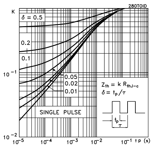
Figure 13. Thermal impedance
