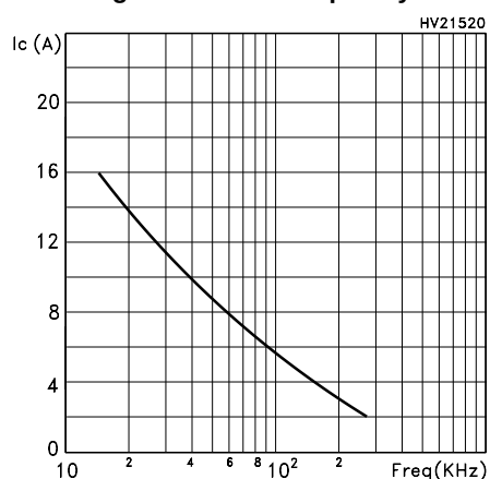
Figure 16: Ic vs frequency
